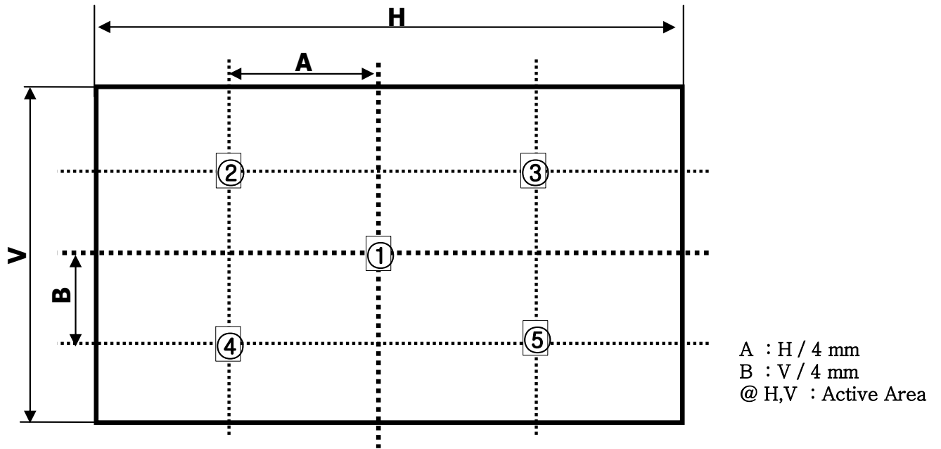
FIG. 2 Measure Point for Luminance
