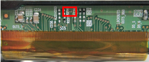
FIG. 3 Measure point
