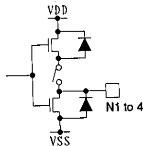
Figure 10 Supply Current Test Circuit
