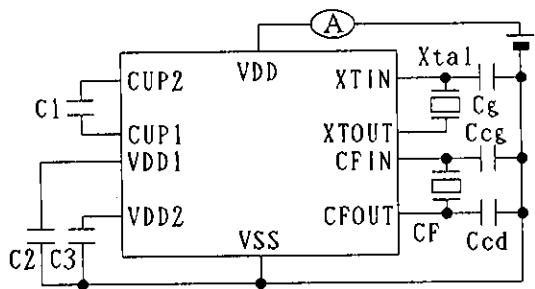
Figure 7 Supply Current Test Circuit
