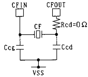
Figure 1-2 Oscillator Circuit (CF pins)
