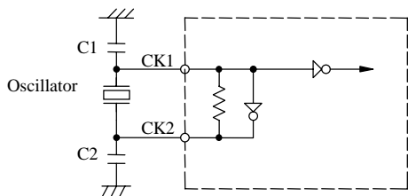
Figure2 Ceramic Oscillation
