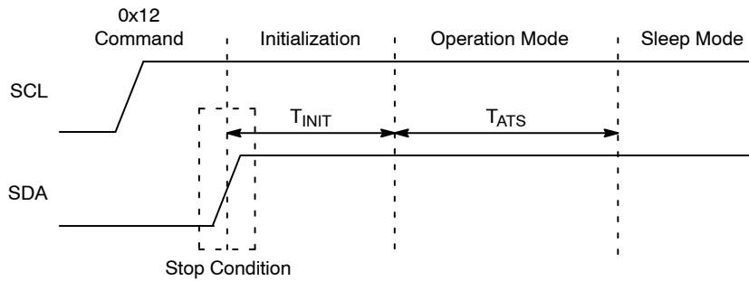
Figure 18. Timing Diagram after 0x12 Command
