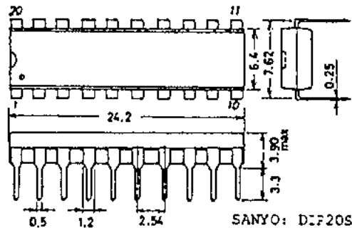
Case Outline 3008A-D20IC (unit:mm)
