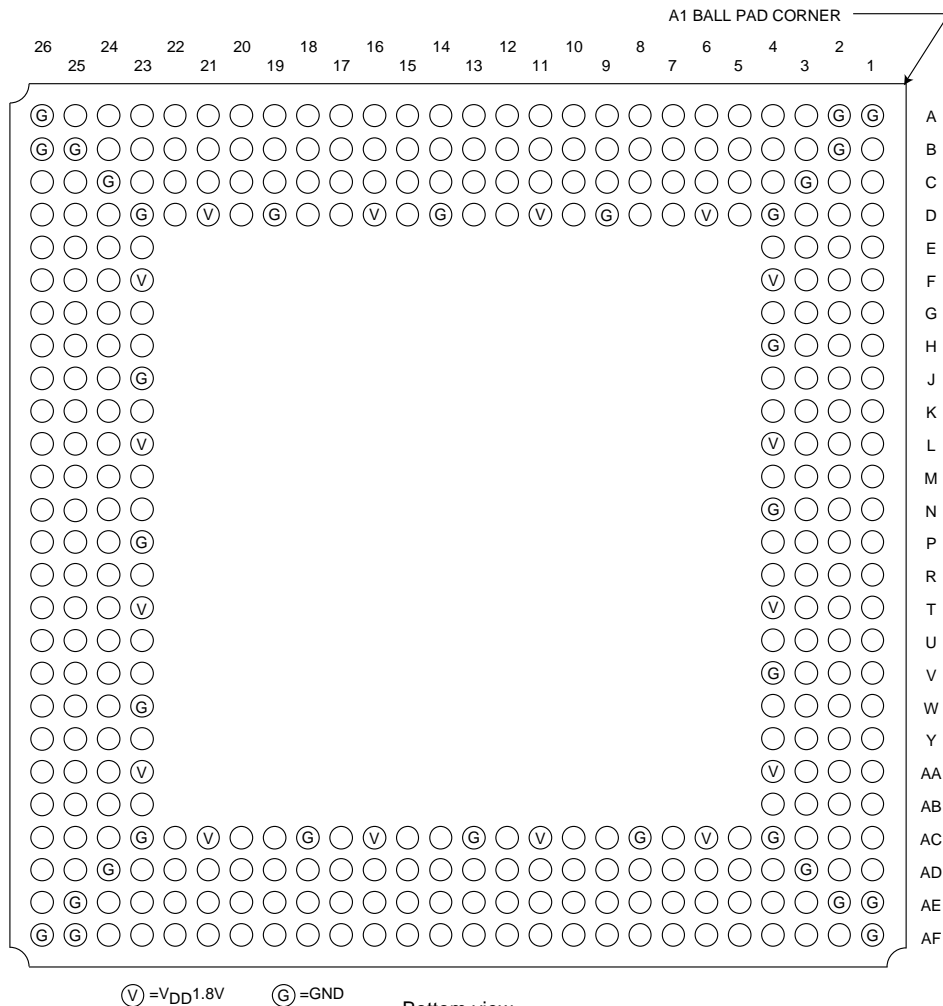
Bottom view 352 SOLDER BALLS
