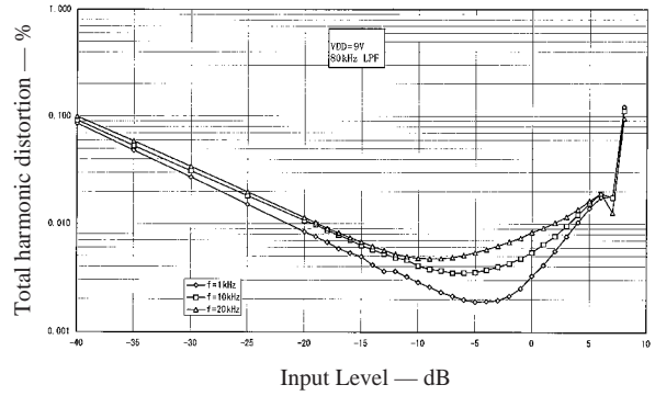
THD – Input Level Characteristics
