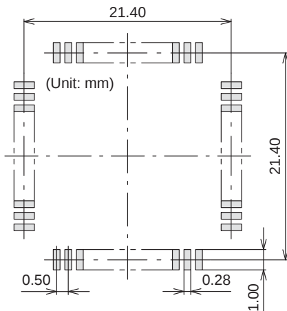
SOLDERING FOOTPRINT*
