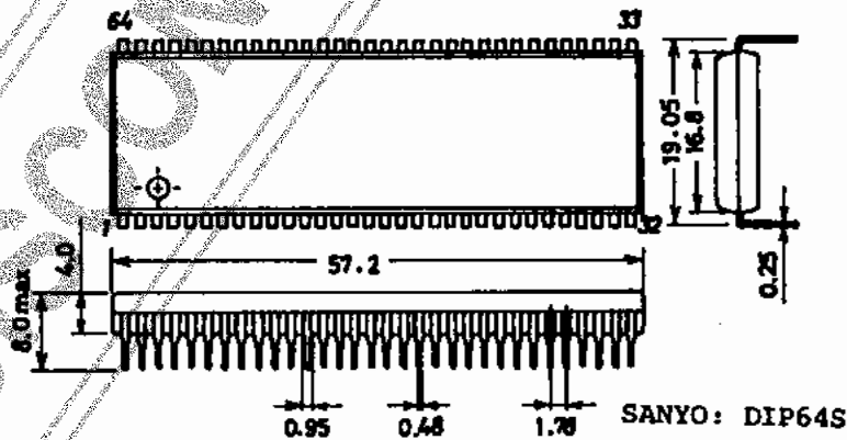
Case Outline 3071-D641C (unit: mm)
