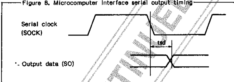
Figure 8. Microcomputer Interface serial output timing
