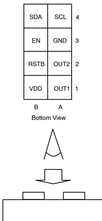
Figure 2. Pin Layout
