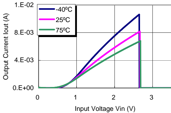
Detector threshold=2.7V
