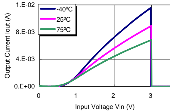
Detector threshold=3.0V
