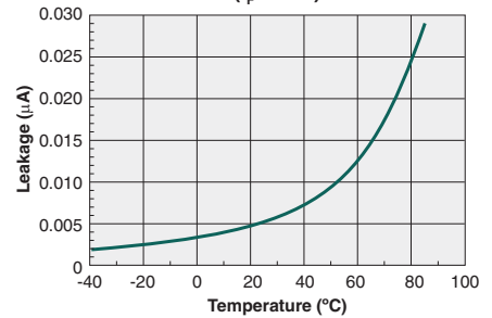
Typical Leakage vs. Temperature Measured Across Pins 4&6 ( I_F=5mA )
