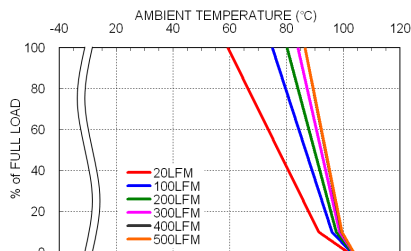
LCD20-48S05 Derating Curve
