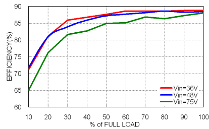
LCD20-48S05 Efficiency vs. Output Load
