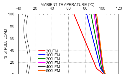
LCD20-48S05 Derating Curve With Heat-sink
