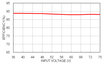
LCD20-48S05 Efficiency vs. Input Voltage
