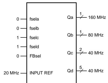
Figure 6. Triple-Frequency Configuration
