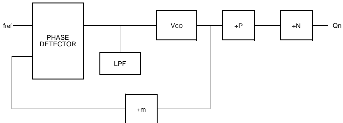
Figure 9. PLL Block Diagram
