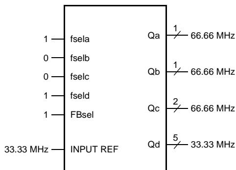
Figure 4. Dual-Frequency Configuration
