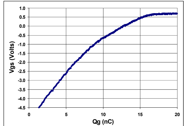
Figure 2 – Gate Charge for V_{DS} = 0.1\text{V}
