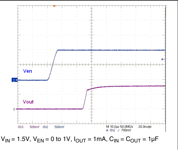
Figure 13. Enable transient
