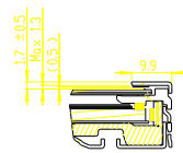
SECTION AA-AA SCALE 1/1
