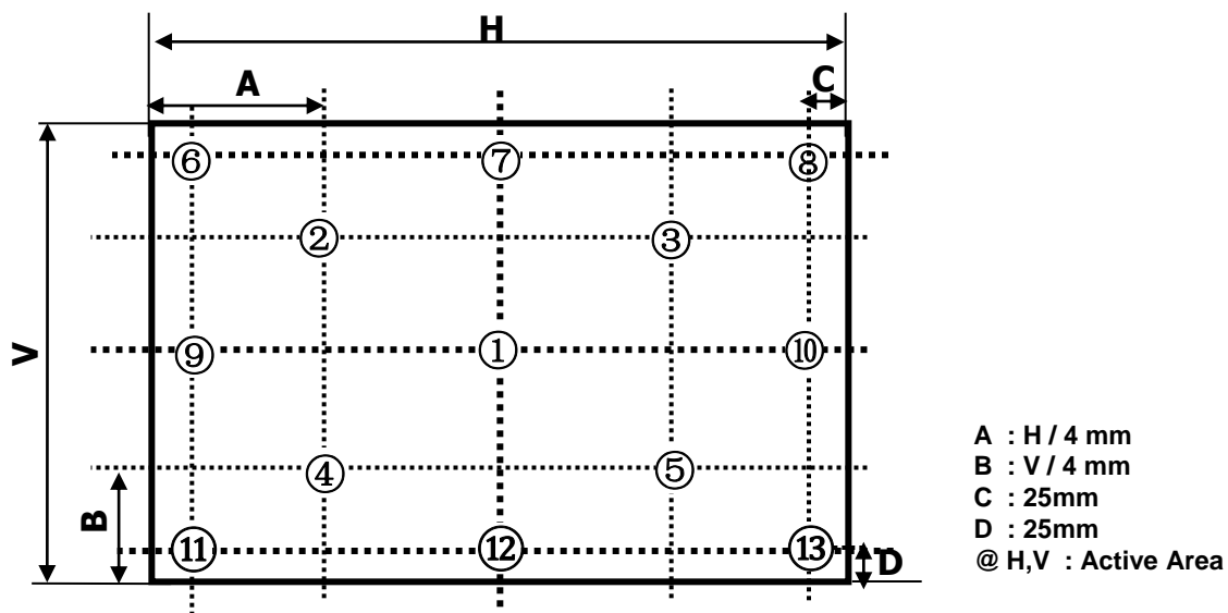
FIG. 2-2 13 Points for Luminance Measure
