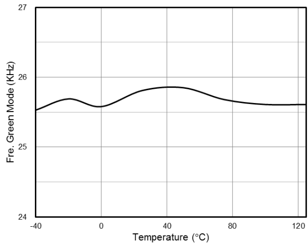
Fig. 4 Fre. Green Mode vs. Temperature
