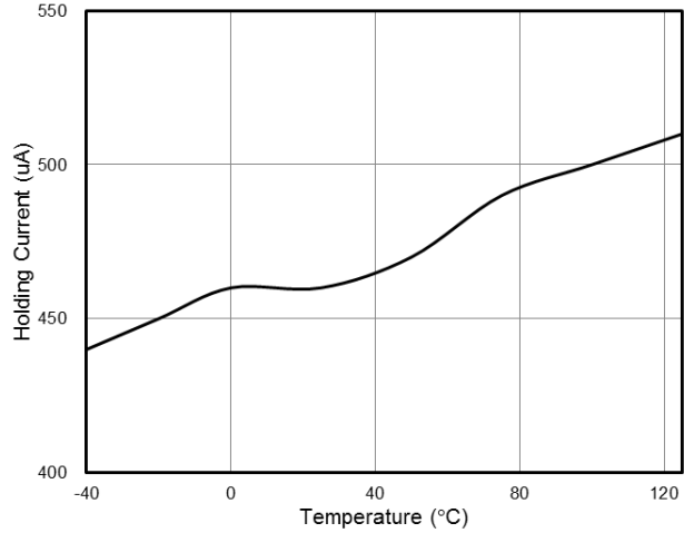
Fig. 2 Holding Current vs. Temperature
