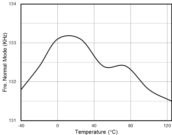
Fig. 3 Fre. Normal Mode vs. Temperature
