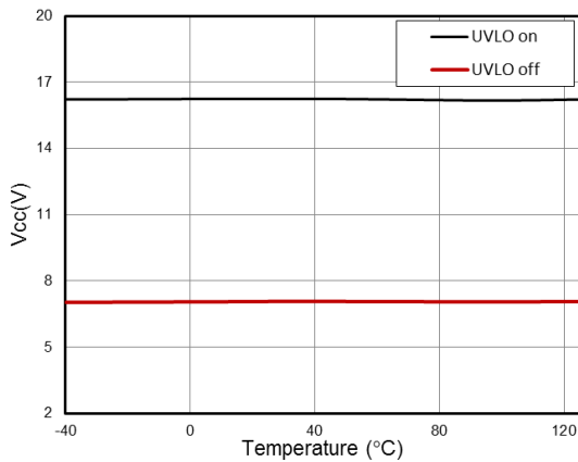
Fig. 5 UVLO level vs. Temperature
