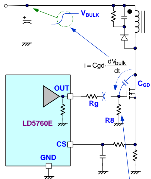
This resistor would protect the MOSFET from being false triggered by the current through C_{GD} , if R_G is disconnected.
