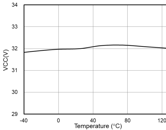
Fig. 4 VCC OVP Level vs. Temperature
