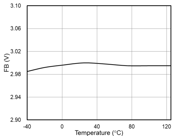
Fig. 7 FB OVP Level vs. Temperature
