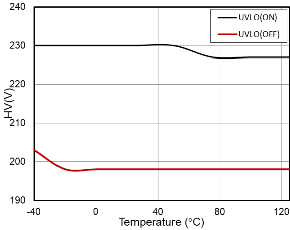
Fig. 2 HVBI/HVBO Level vs. Temperature
