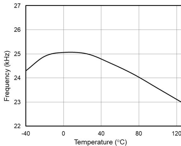
Fig. 6 Frequency Green Mode vs. Temperature
