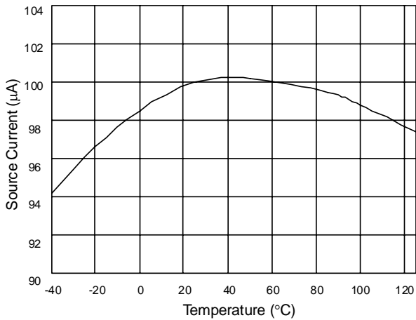
Fig. 15 (-) Latch Pin Source Current vs. Temperature
