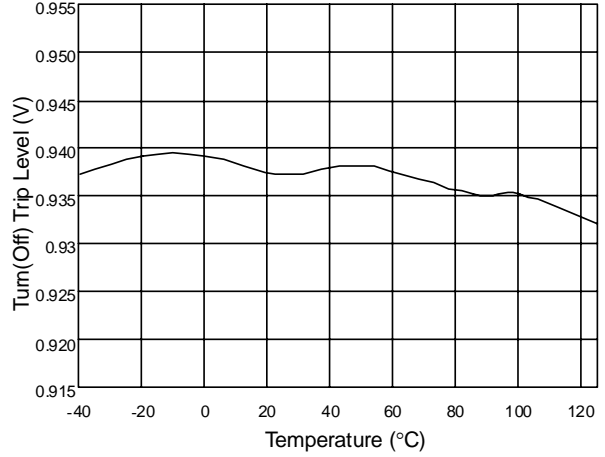
Fig. 14 Latch Pin Turn(Off) Level vs. Temperature
