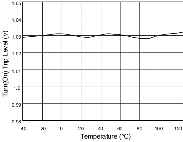
Fig. 13 Latch Pin Turn(On) Level vs. Temperature
