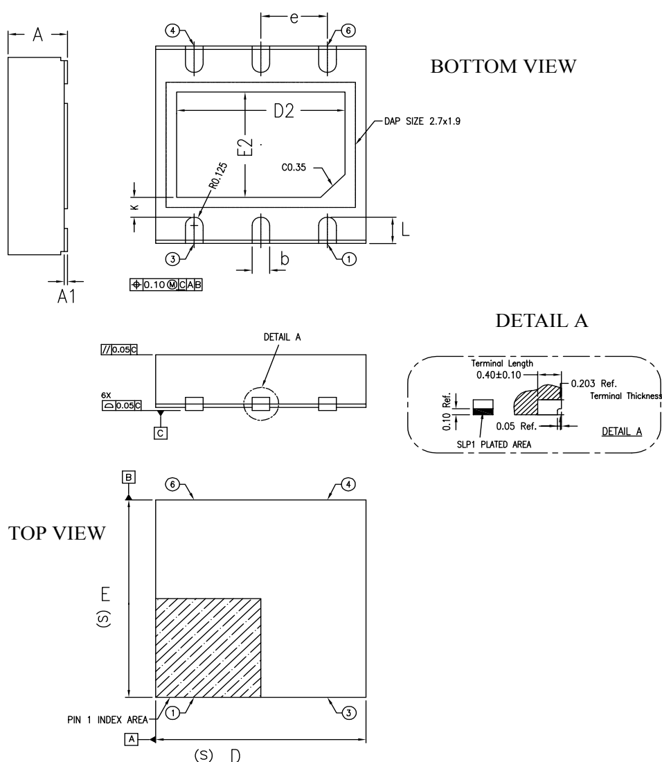
Figure 40. DFN6 (3x3) package outline
