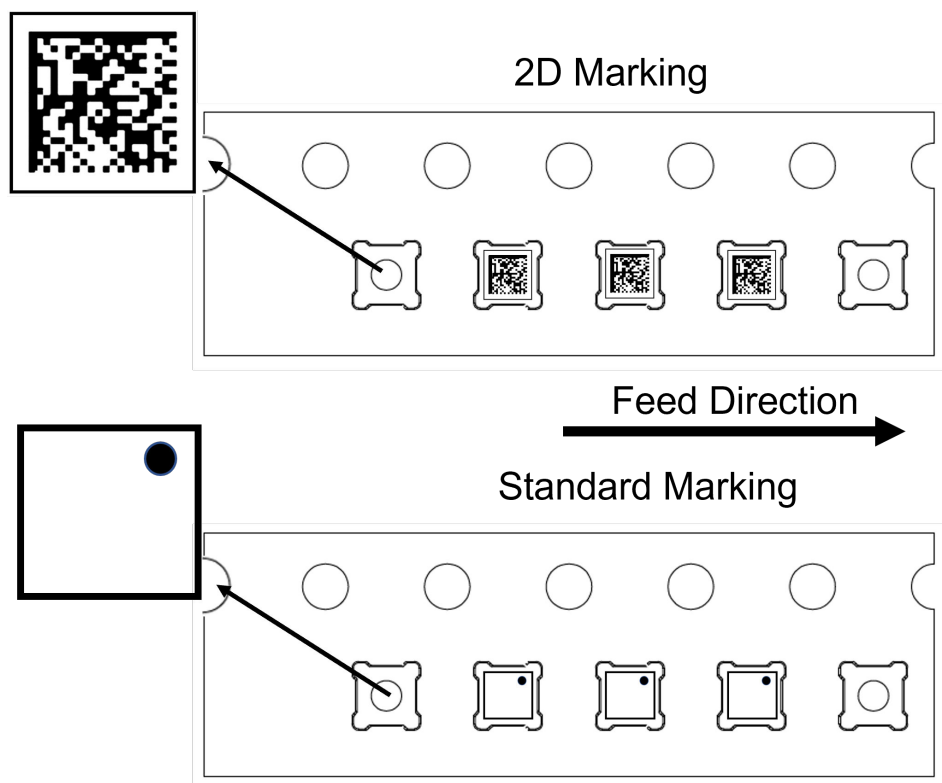
Figure 33. Pin 1 orientation
