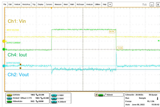
Figure 21. Load transient
