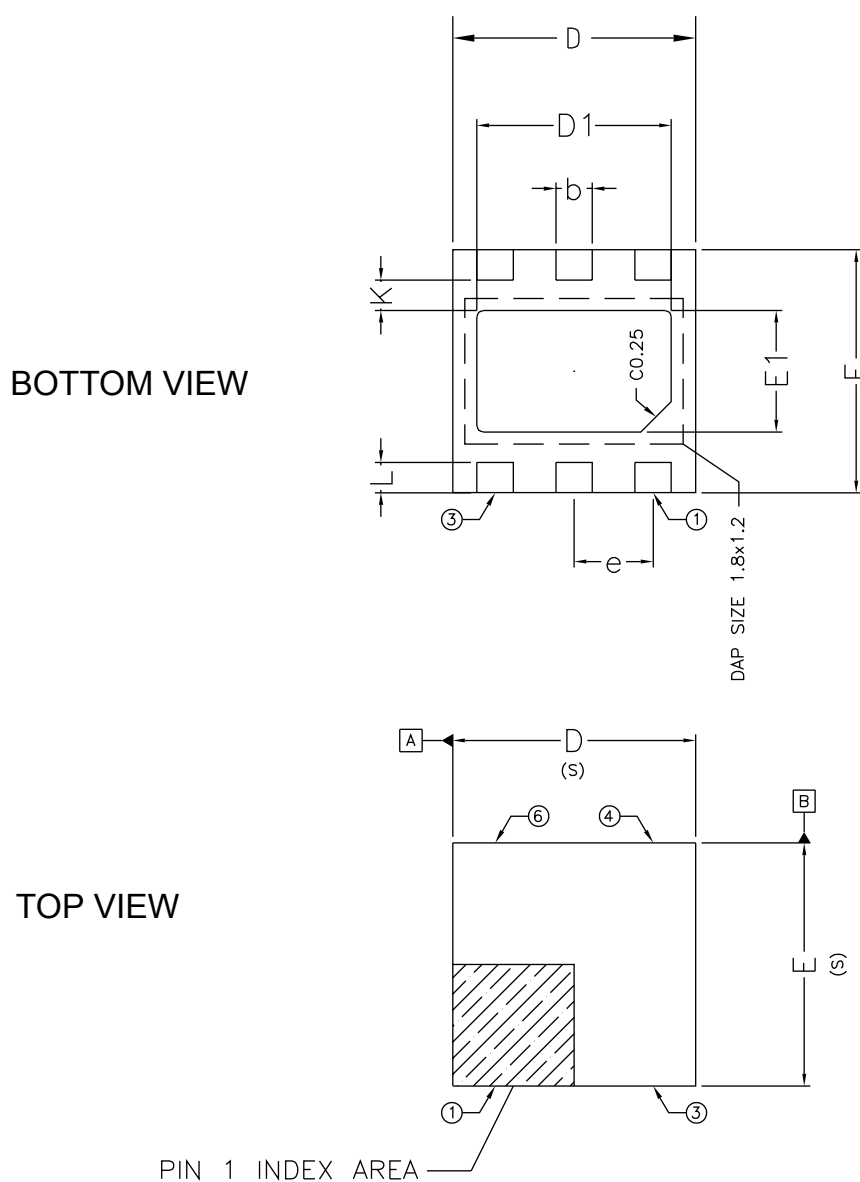
Figure 24. DFN6 (2 x 2) package outline
