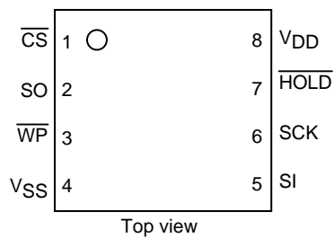
Figure 1 Pin Assignments
