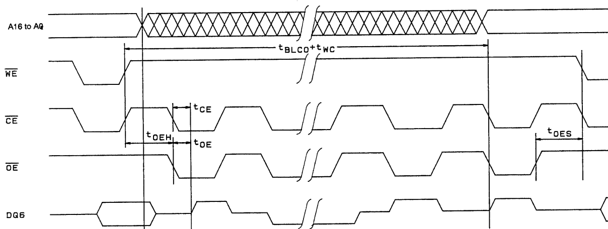
Figure 5 Toggle Bit
