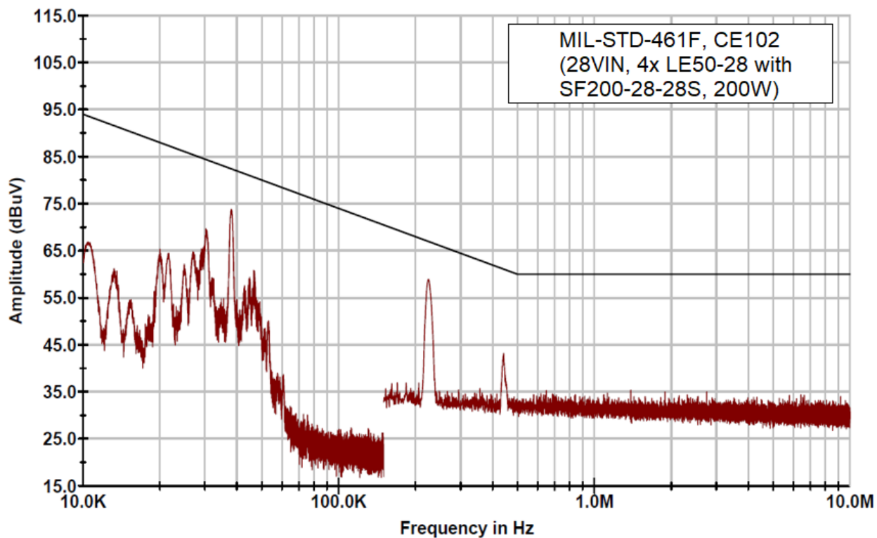
Figure 7-2. LE50-28 EMI
