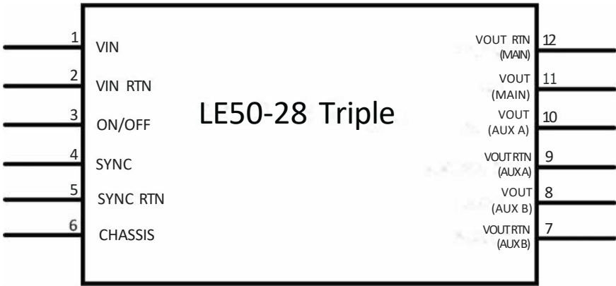
Figure 8-1. LE50-28 Triple Pin Configuration
