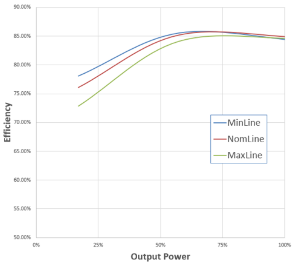
Figure 7-1. LE50-28 Efficiency
