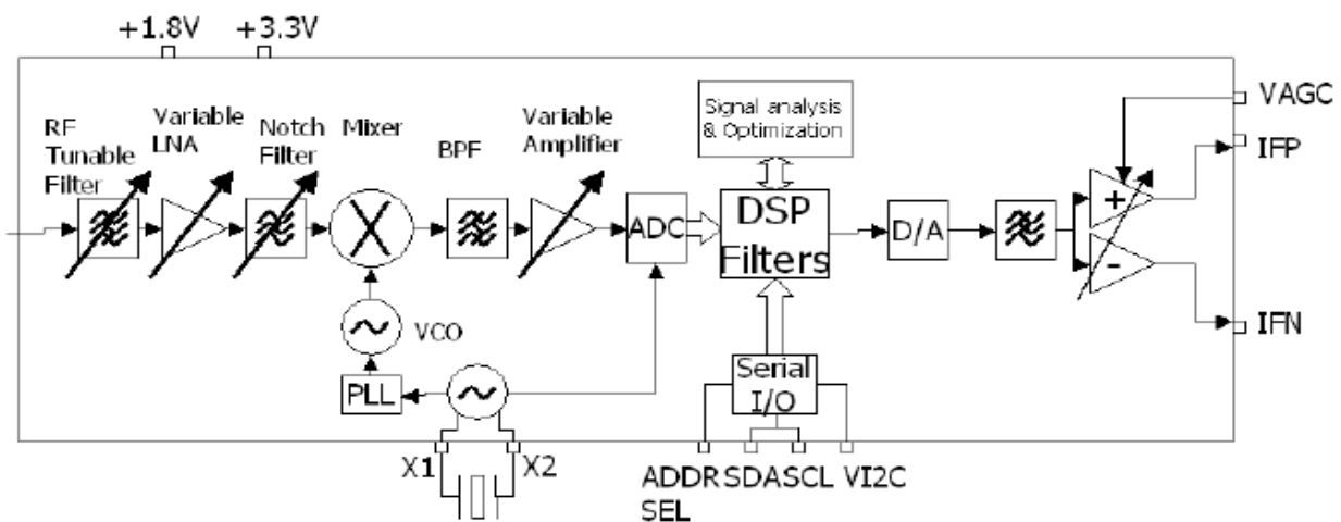
Figure 1. XC5200C Block Diagram
