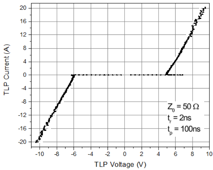
Fig5.TLP Measurement
