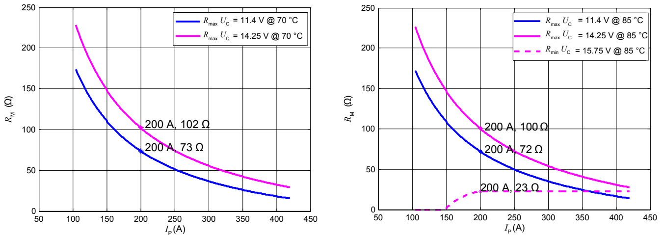
Figure 1: Maximum measuring resistance
