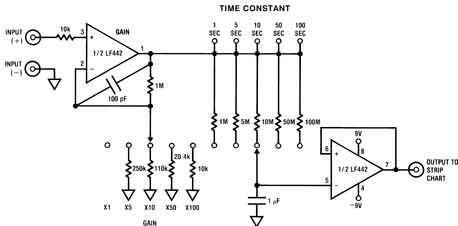
Battery Powered Strip Chart Preamplifier
