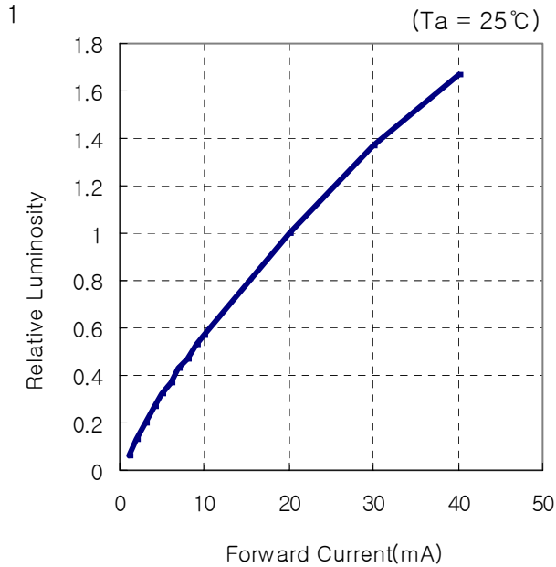
(1) Relative Luminous Intensity vs Forward Current (IF-Iv)
