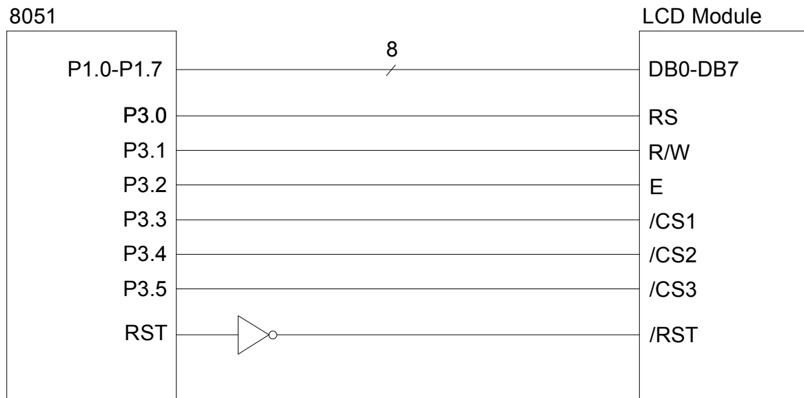
b. Application Circuit 2
