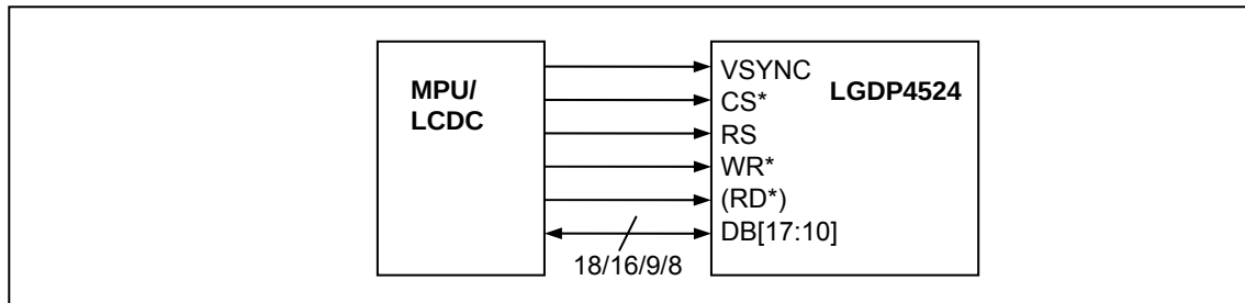
Figure 33: VSYNC interface
