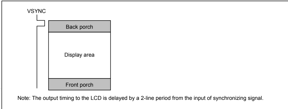
Figure 11 Back/front porches
