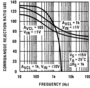
Common-Mode Rejection
