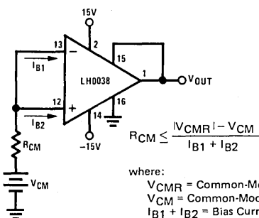
FIGURE 9. Bias Current Return
