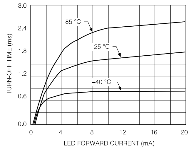
F. Turn-off Time vs. LED Current
