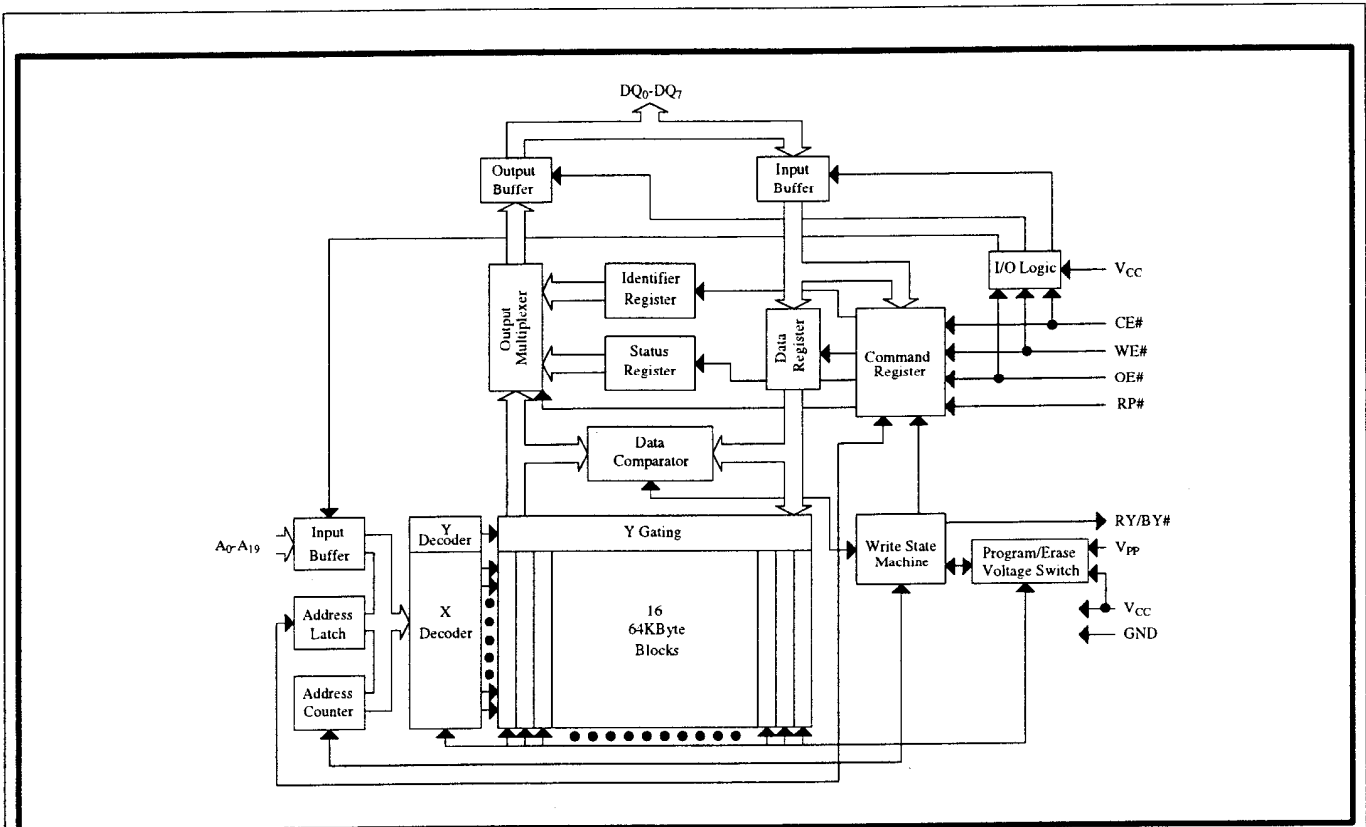
Figure 1. Block Diagram
