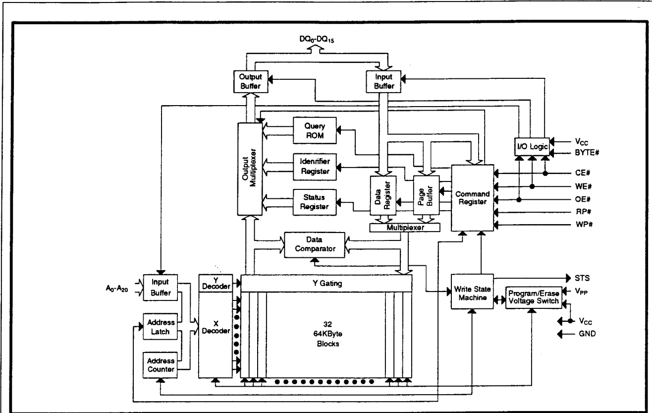
Figure 1. Block Diagram
