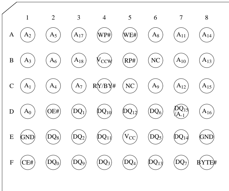
Figure 2. CSP 48-Ball Pinout
