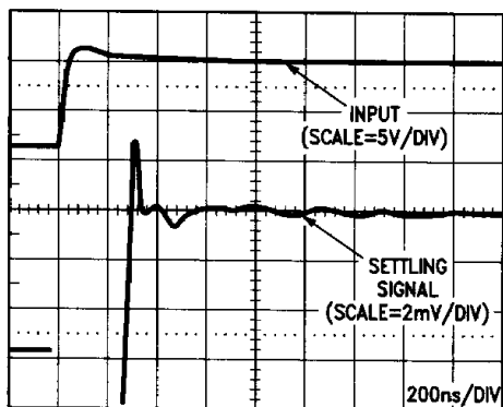
Settling Signal
