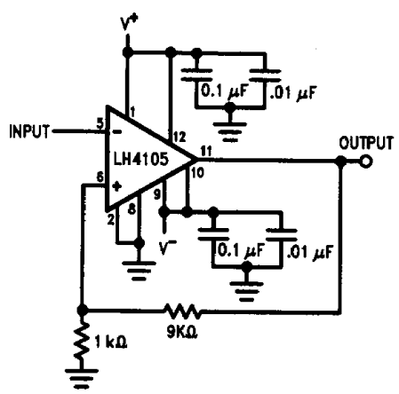
FIGURE 5. 10X Buffer Amplifier
