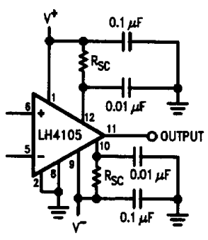
FIGURE 3. Using Resistor Current Limiting
