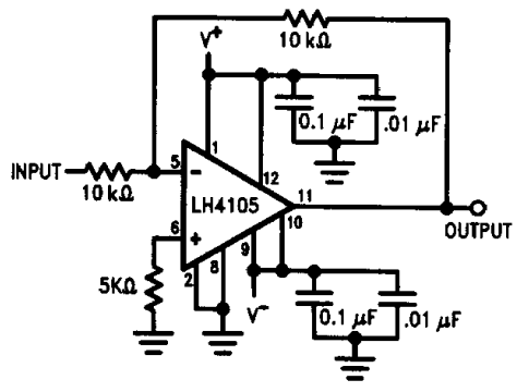
FIGURE 6. Unity Gain Inverter
