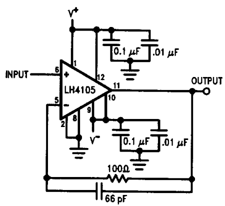
FIGURE 4. Unity Gain Follower
