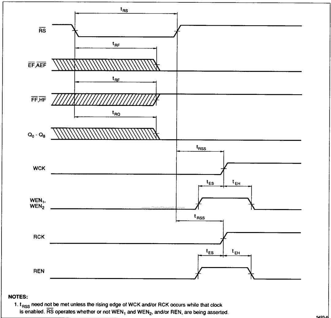
Figure 7. Reset Timing
