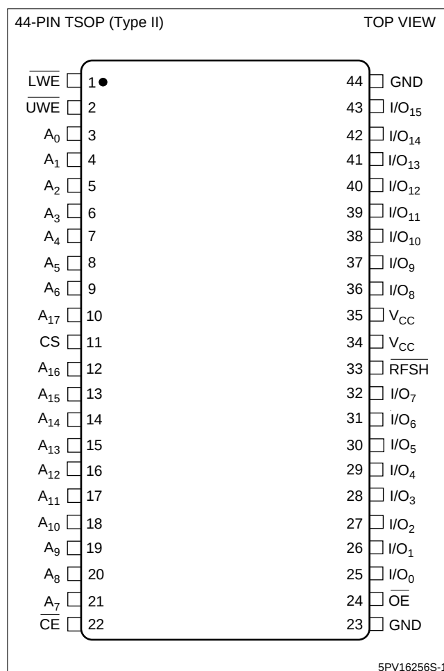
Figure 1. Pin Connections
