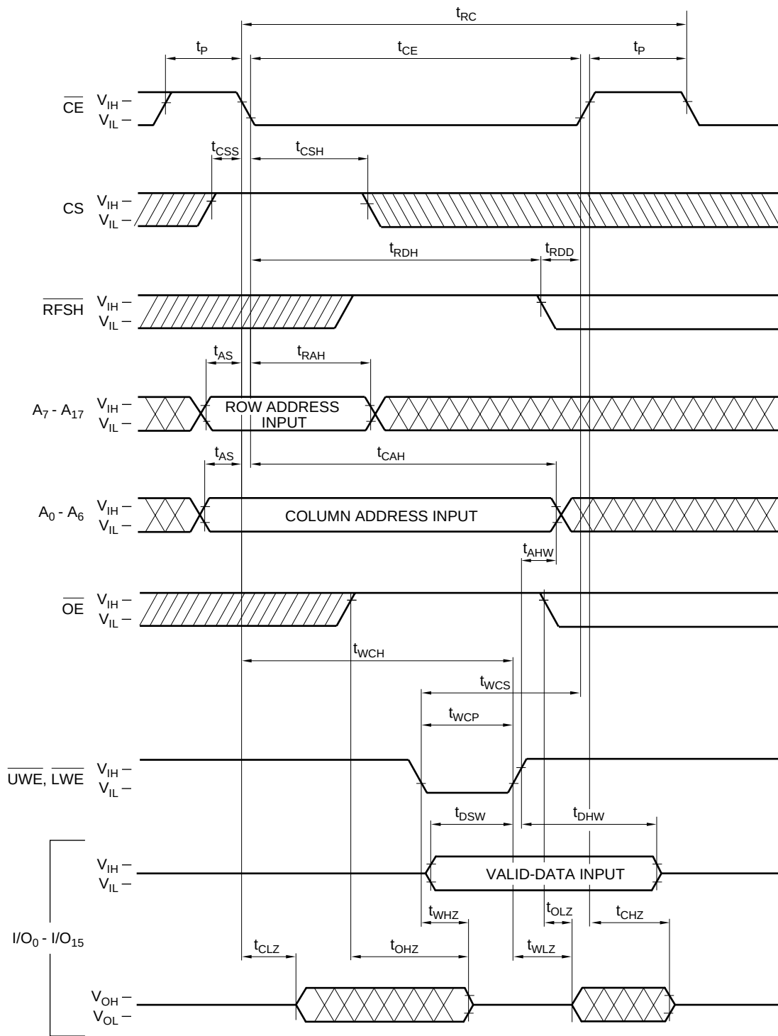
Figure 5. Write Cycle (1) (OE Clock)
