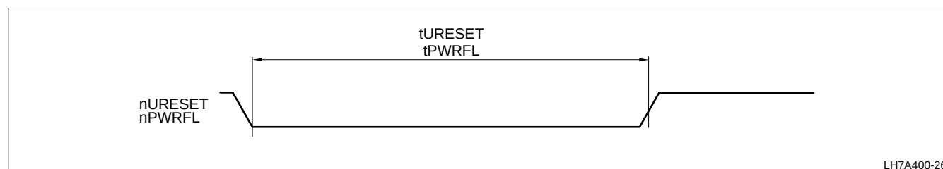
Figure 43. External Reset
