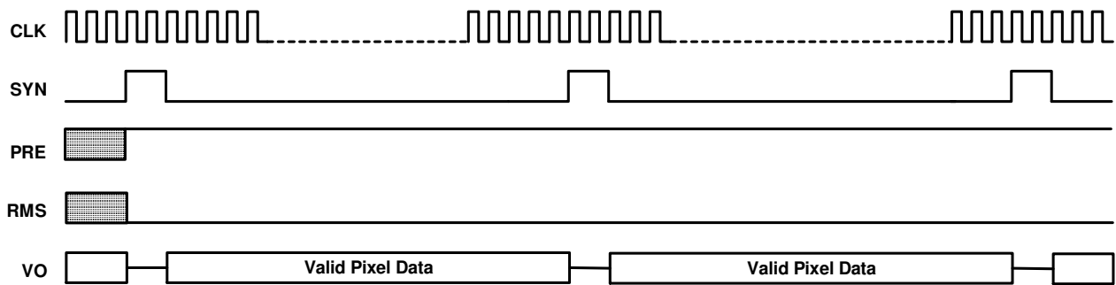
Figure 7: Frame Mode Destructive Read with External Reset Timing
