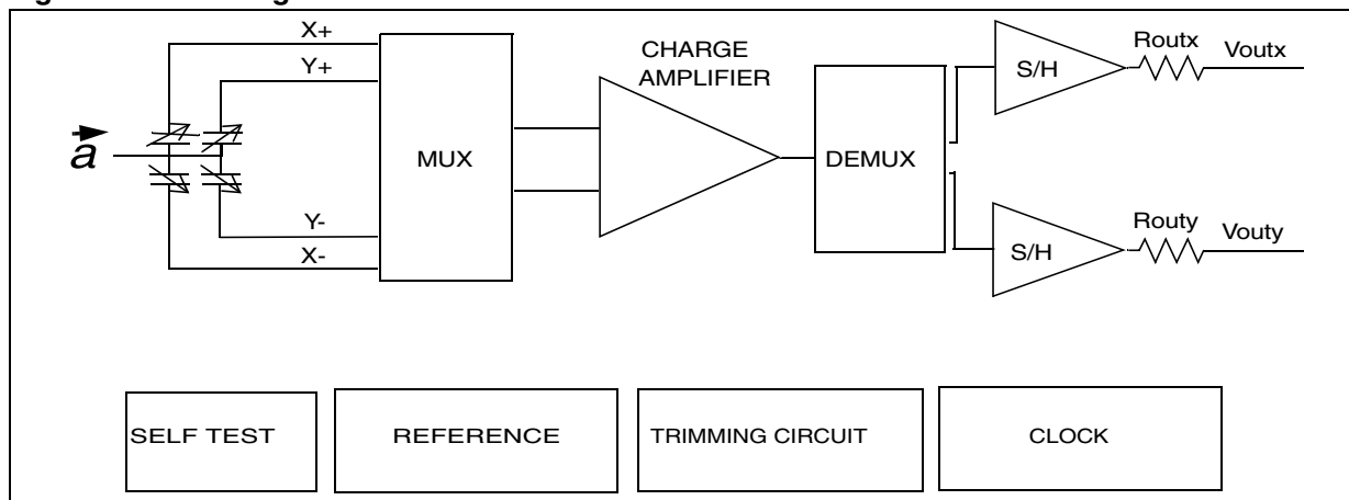
Figure 2. Block Diagram
