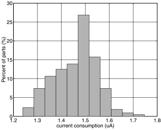
Figure 16. Current consumption in power down mode at 3.3V
