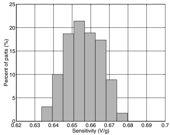
Figure 8. X axis Sensitivity at 3.3V
