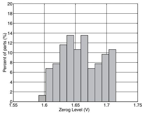
Figure 6. X axis Zero g Level at 3.3V
