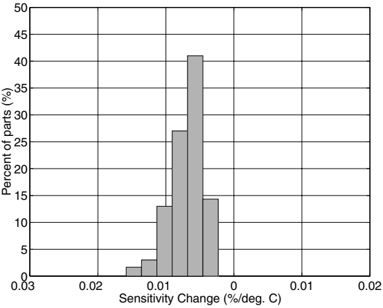
Figure 13. Y axis Sensitivity Change Vs. Temperature
