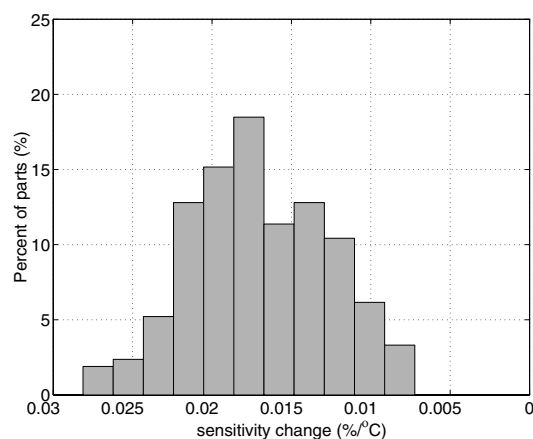
Figure 16. z-axis sensitivity change vs. temperature
