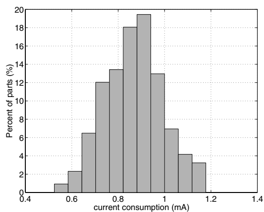
Figure 20. Current consumption in power down mode at 3.3V
