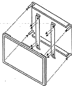
Figure of Shock test's jig Module fixed position ( M4 Bolt×16 )
