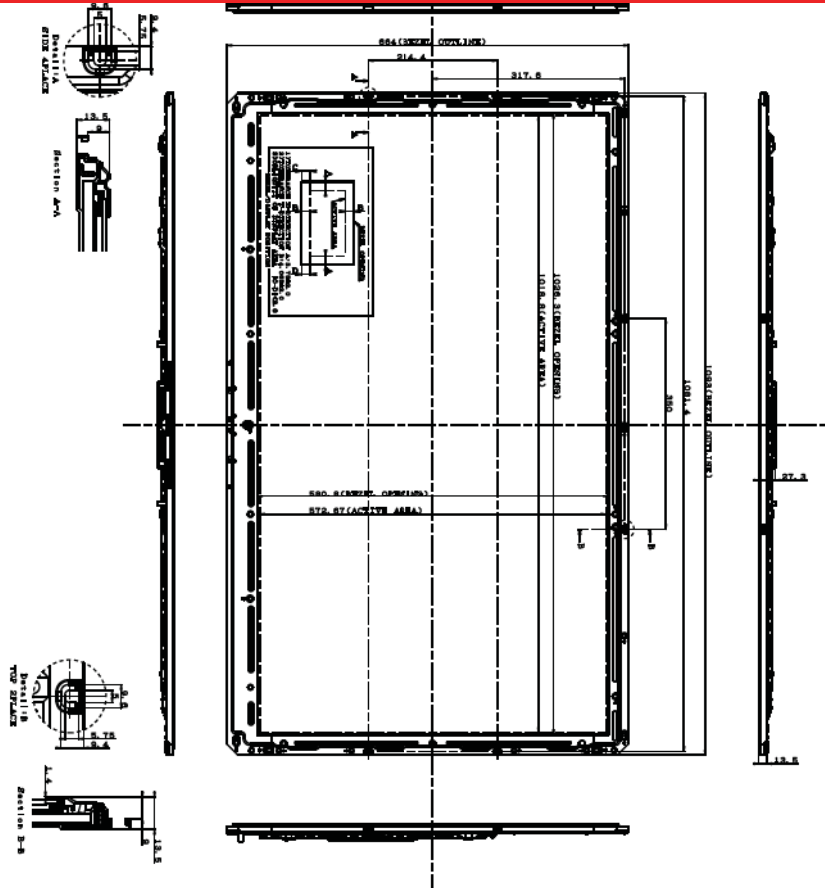
Fig.17 TFT-LCD MODULE OUTLINE DIMENSIONS
