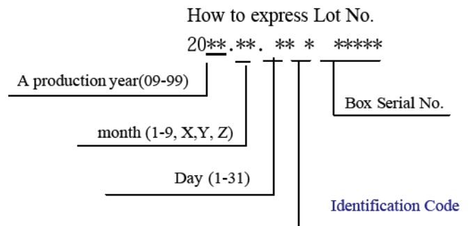
Fig.15 Packing label description specification
